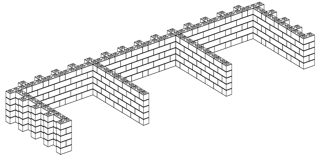
ISOMETRIC VIEW
